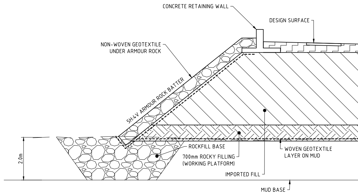
TYPICAL REVETMENT WALL DETAIL
